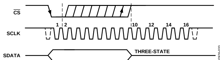
Figure 20. Entering Power-Down Mode
