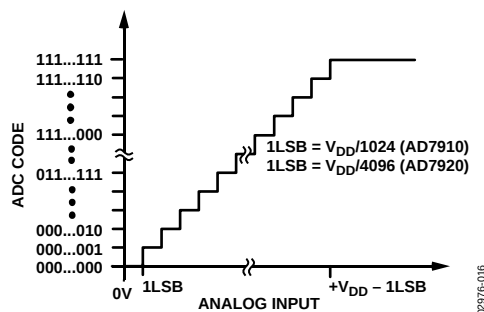
Figure 16. Transfer Characteristic
