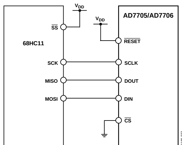
Figure 22. AD7705/AD7706-to-68HC11 Interface
