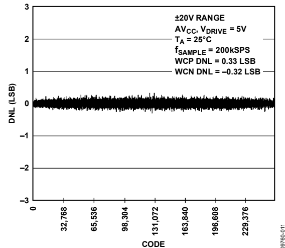
Figure 12. Typical DNL, \pm 20V Range
