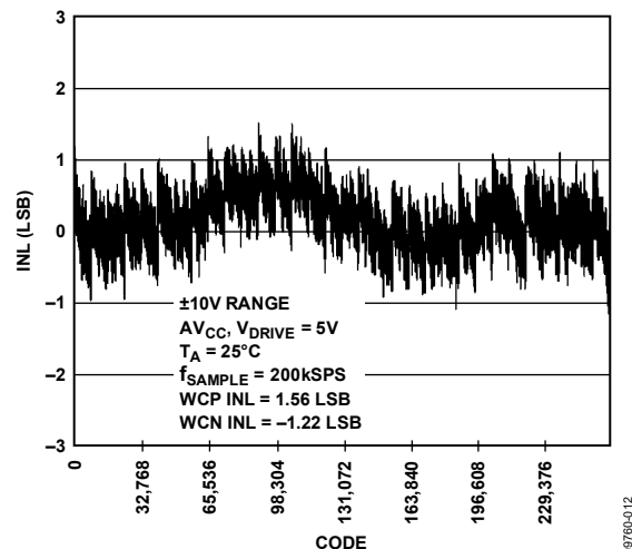
Figure 13. Typical INL, \pm 10V Range
