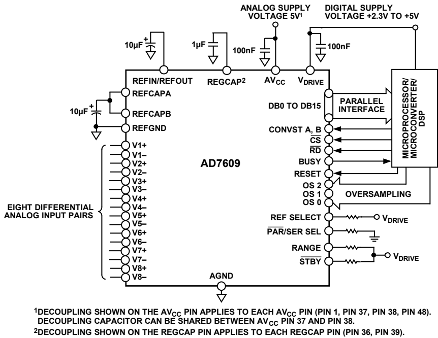
Figure 41. Typical Connection Diagram
