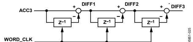
Figure 27. Differentiator
