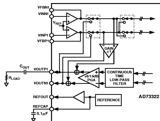
Figure 36. Example Circuit for Single-Ended Output
