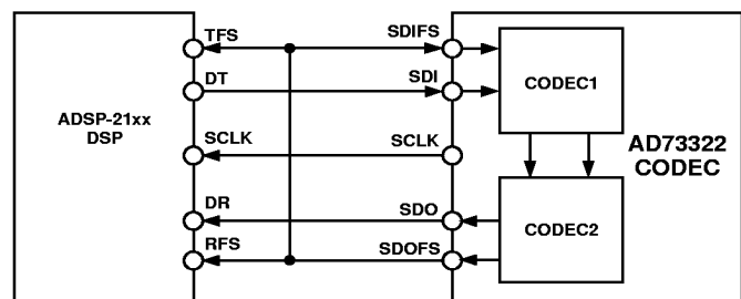
Figure 19. Directly Coupled or Frame Sync Loop-Back Configuration
