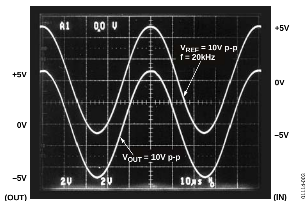
Figure 3. Rail-to-Rail Reference Input to Output at 20 kHz
