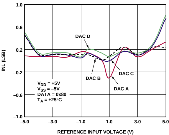
Figure 13. INL vs. Reference Input Voltage
