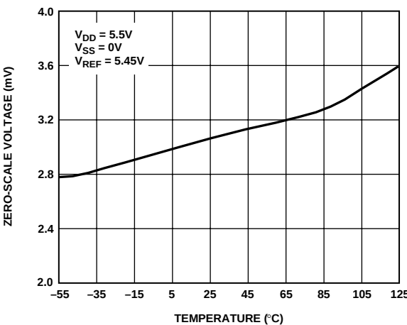
Figure 15. Zero-Scale Voltage vs. Temperature
