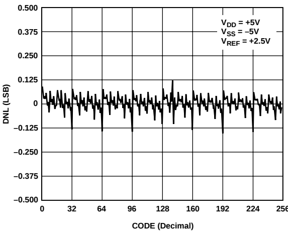
Figure 14. DNL vs. Code
