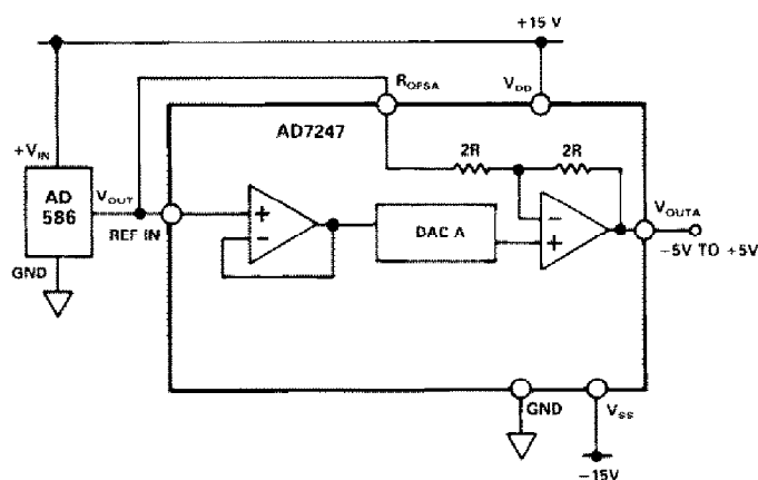
Figure 9. Bipolar Configuration
