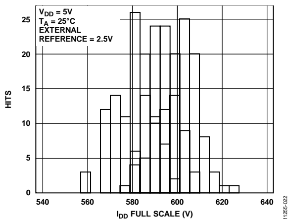
Figure 22. I_{DD} Histogram
