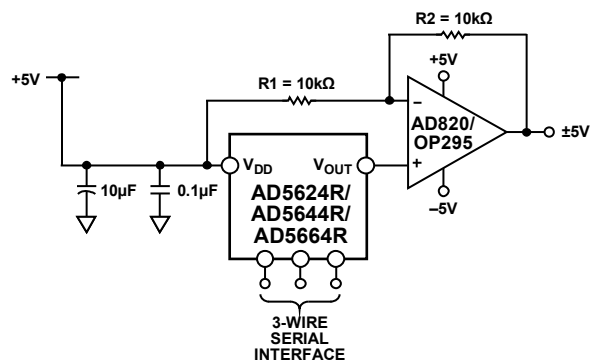
Figure 63. Bipolar Operation with the AD5624R/AD5644R/AD5664R
