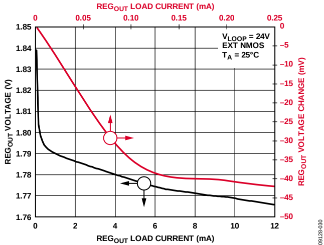
Figure 31. REG_OUT Voltage vs. Load Current
