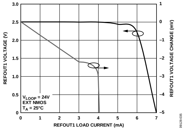
Figure 36. REFOUT1 Voltage vs. Load Current
