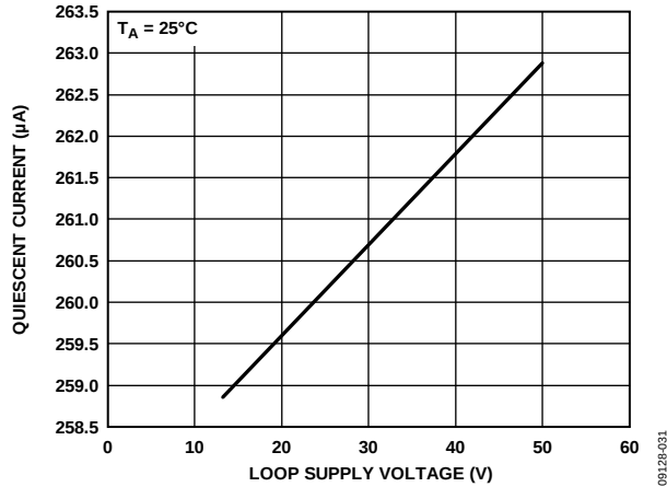
Figure 32. Quiescent Current vs. Loop Supply Voltage
