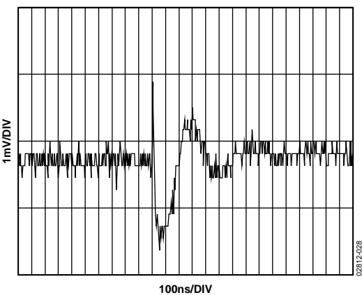
Figure 26. DAC-to-DAC Crosstalk
