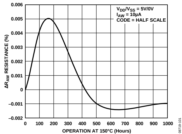
Figure 19. Long-Term Drift Accelerated Average by Burn-In
