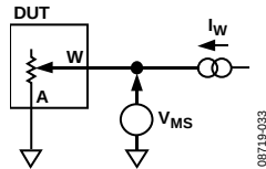
Figure 20. Resistor Position Nonlinearity (Rheostat Operation; R-INL, R-DNL)
