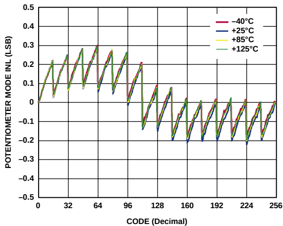
Figure 7. INL vs. Code vs. Temperature, V_{DD} = 5 V
