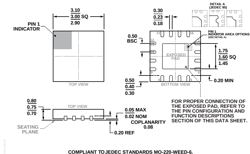
Figure 47. 16-Lead Lead Frame Chip Scale Package [LFCSP] 3 mm x 3 mm Body and 0.75 mm Package Height (CP-16-22) Dimensions shown in millimeters
