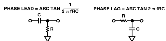
Figure 10. Phase Shift Circuits
