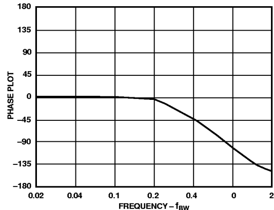
Figure 7. AD2S81A/AD2S82A Phase Plot
