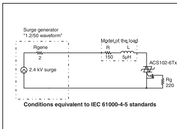
Figure 17. Overvoltage ruggedness test circuit for resistive and inductive loads
