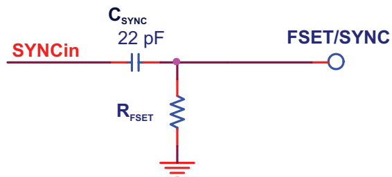
Figure 2: FSET/SYNC AC-Coupling
