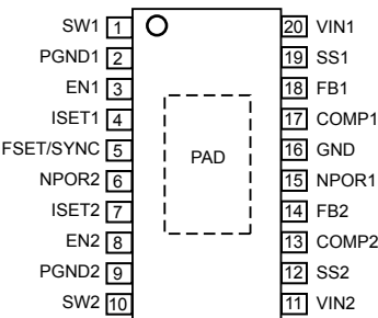
Package LP, 20-Pin TSSOP with Exposed Thermal Pad Pinout Diagram
