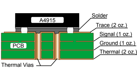
ET Package Schematic Corresponding to Typical PCB Layout
