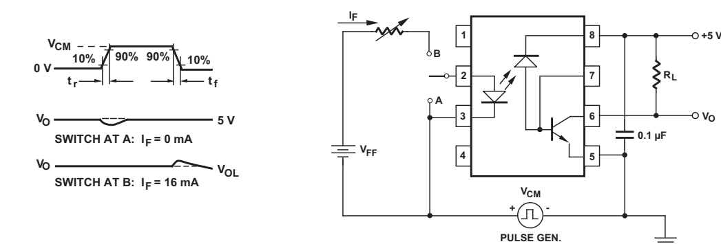
Figure 12: Test Circuit for Transient Immunity and Typical Waveforms
