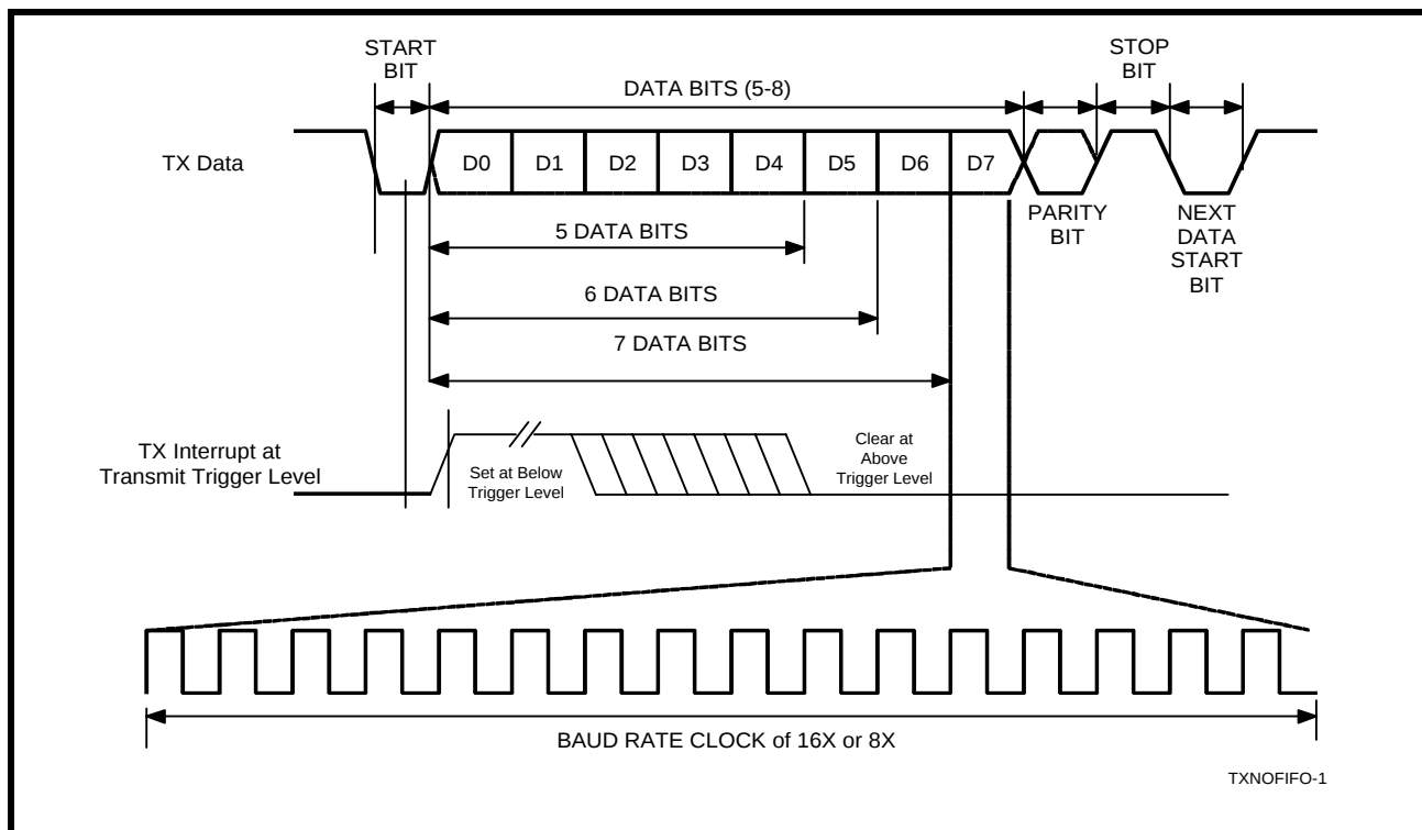
FIGURE 24. TRANSMIT DATA INTERRUPT AT TRIGGER LEVEL
