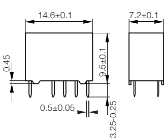
THT version
