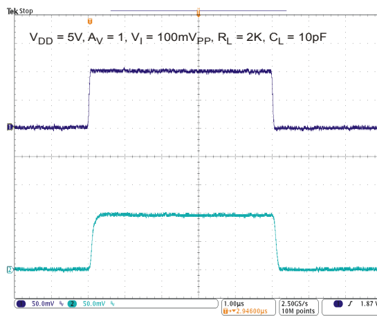
Figure 23 Voltage Follower Small Signal Pulse Response
