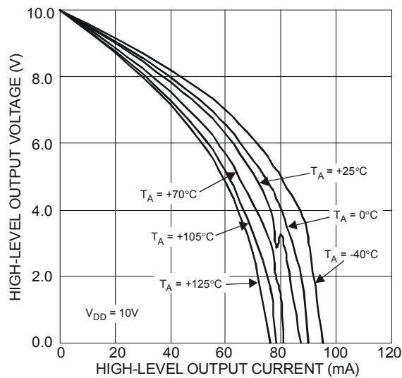
Figure 10 High-Level Output Voltage vs. High-Level Output Current
