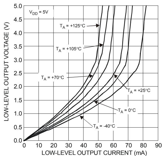
Figure 12 Low-Level Output Voltage vs. Low-Level Output Current
