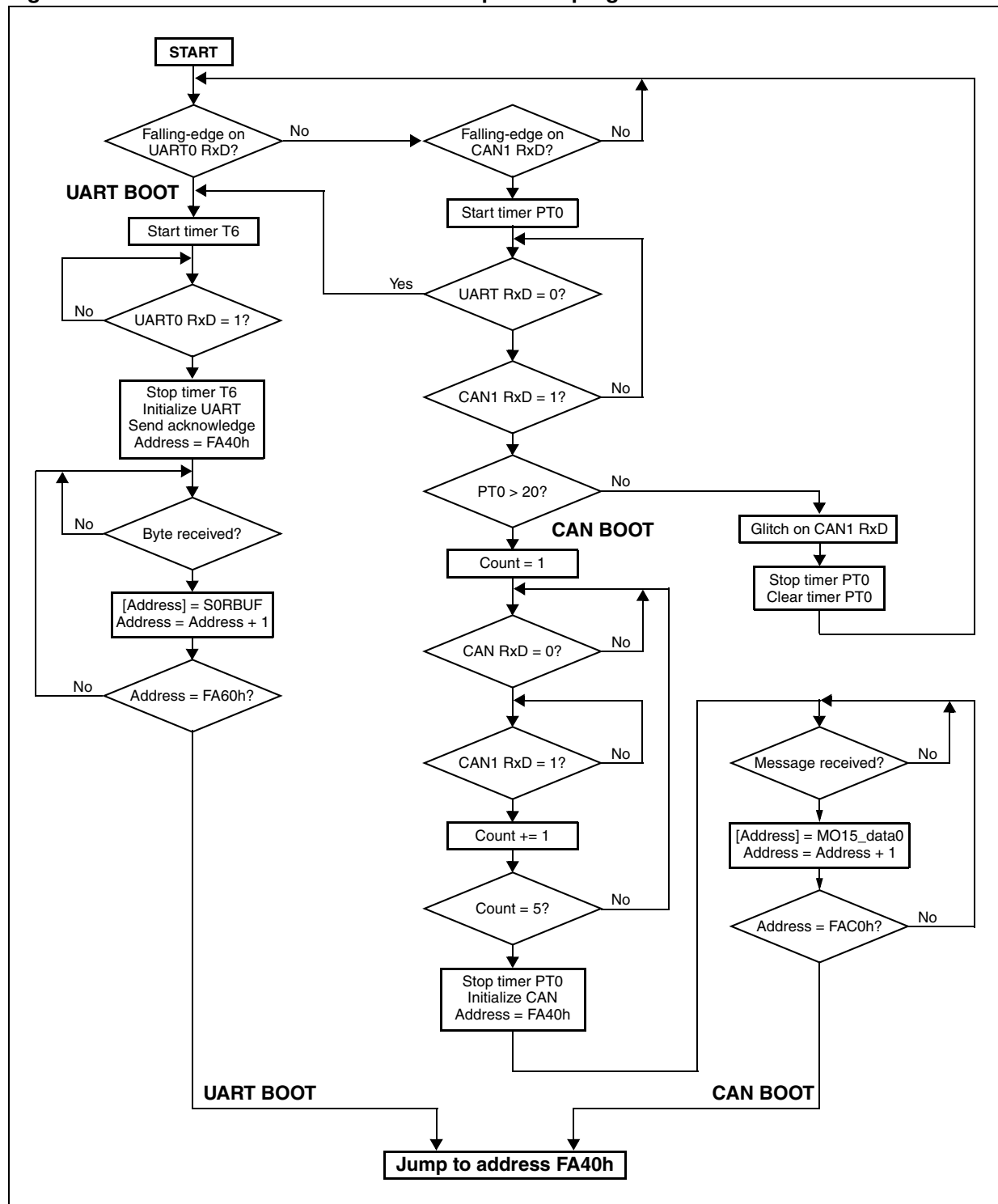
Figure 5. ST10F276E new standard bootstrap loader program flow
