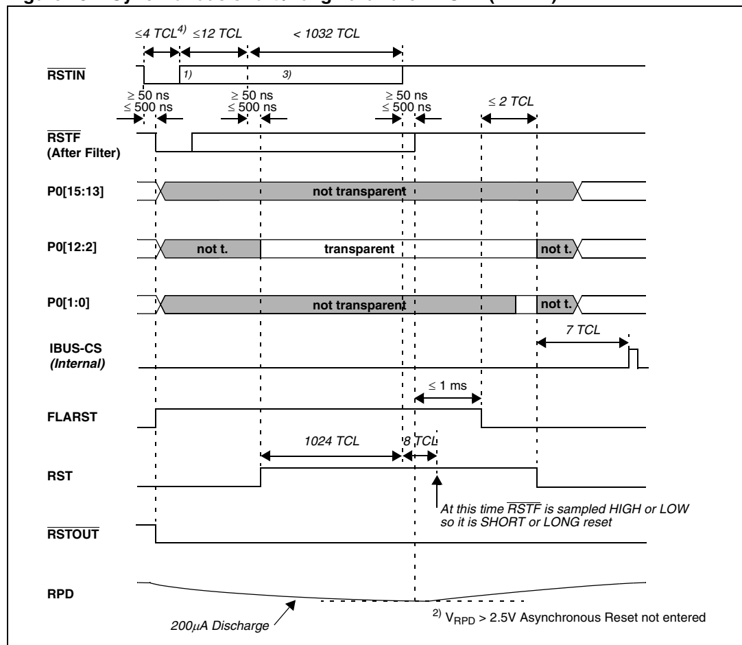
Figure 28. Synchronous short / long hardware RESET ( \overline{\text{EA}} = 1 )
