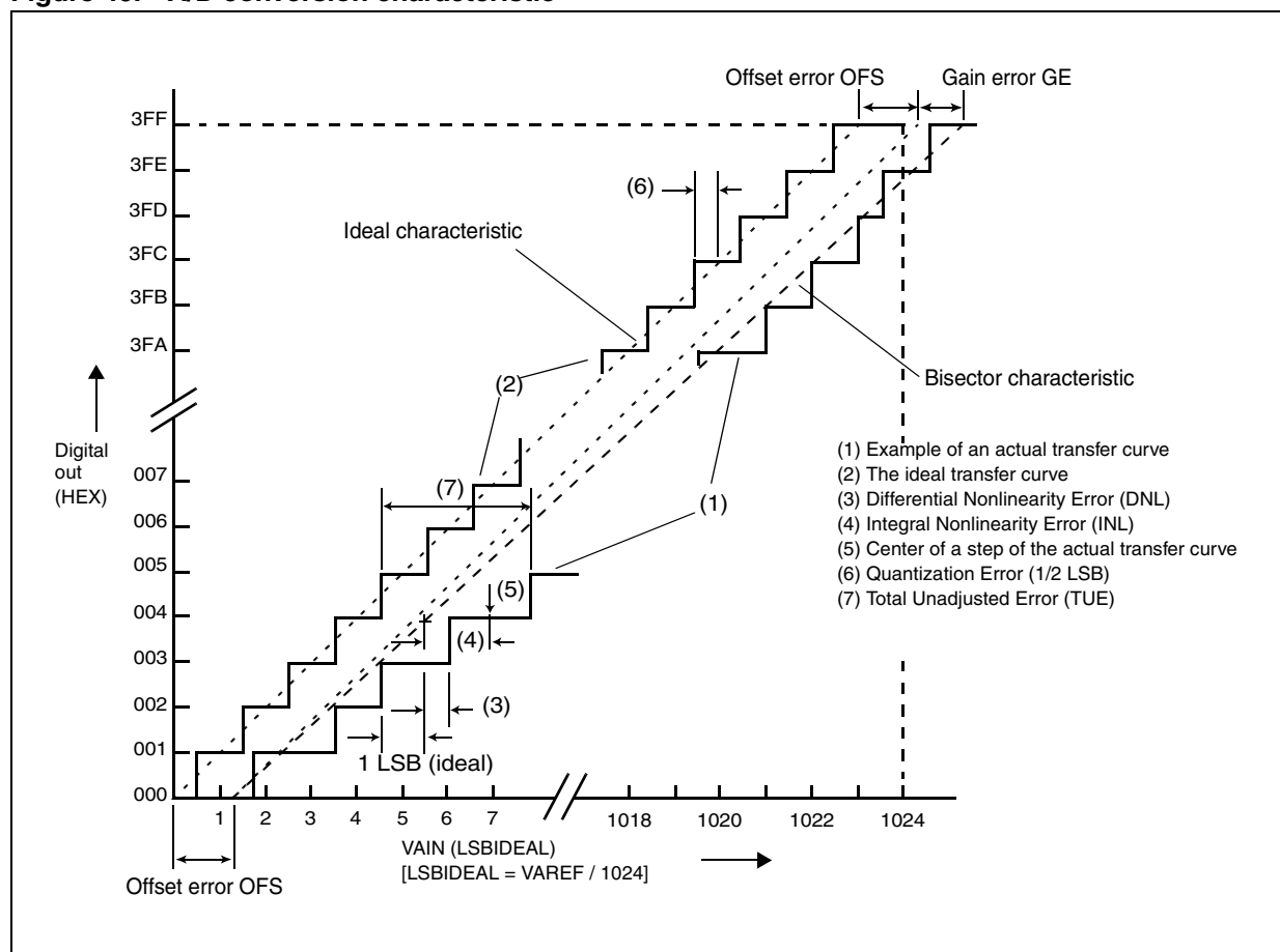
Figure 46. A/D conversion characteristic
