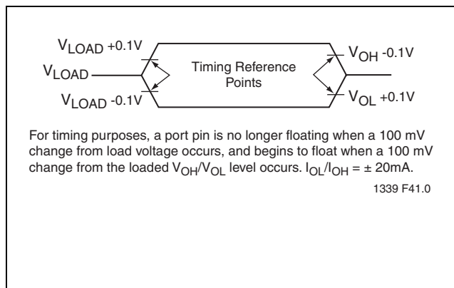
FIGURE 14-8: Float Waveform
