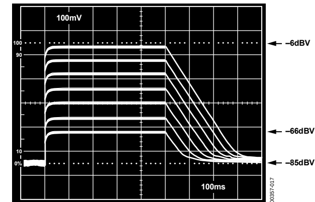
Figure 17. RMS Level Detector Performance with C_{AVG} = 2.2 \mu\text{F}
