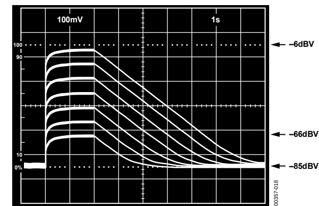
Figure 18. RMS Level Detector Performance with C_{AVG} = 22 \mu\text{F}
