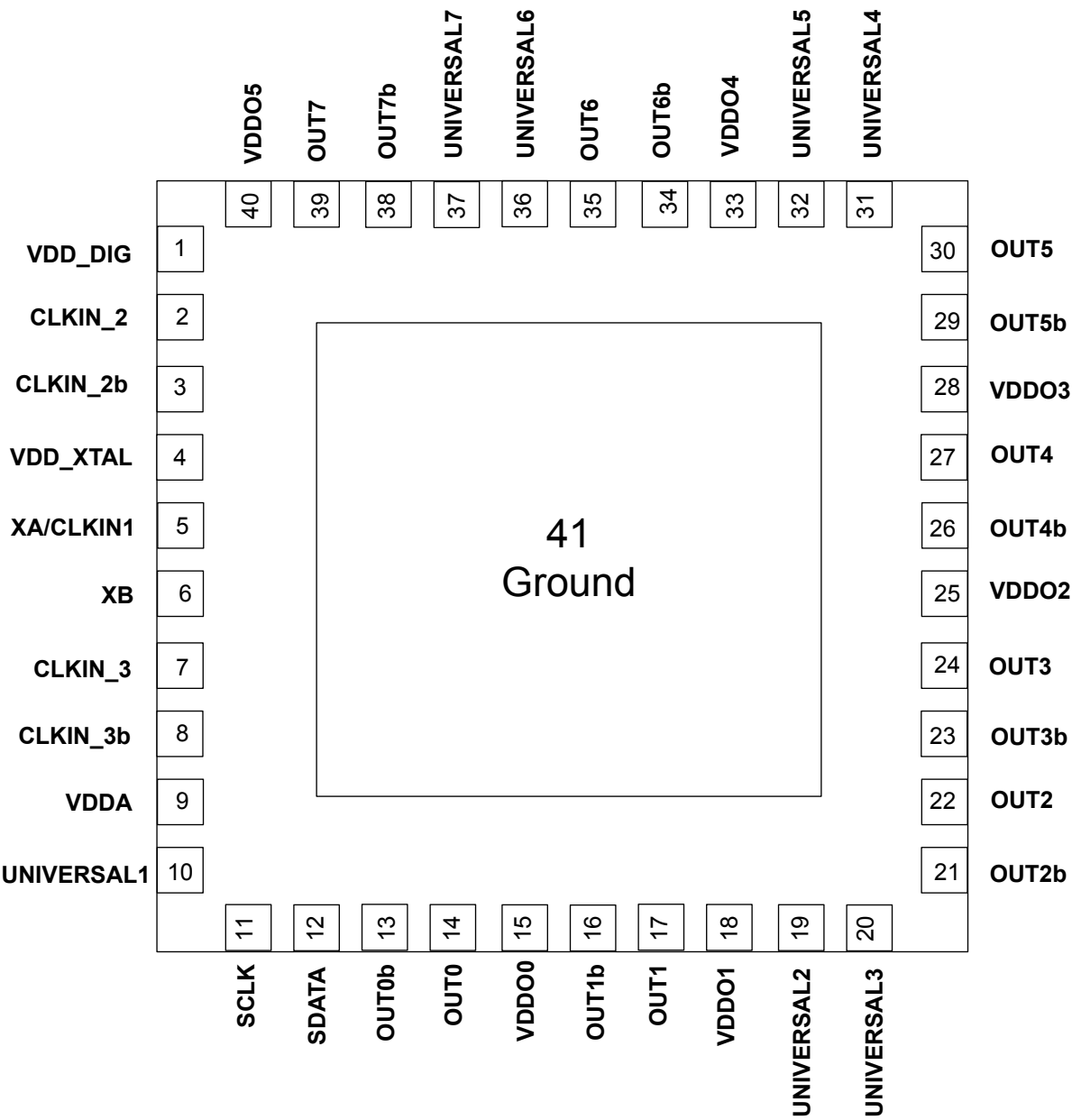
Figure 6.2. 40-QFN
