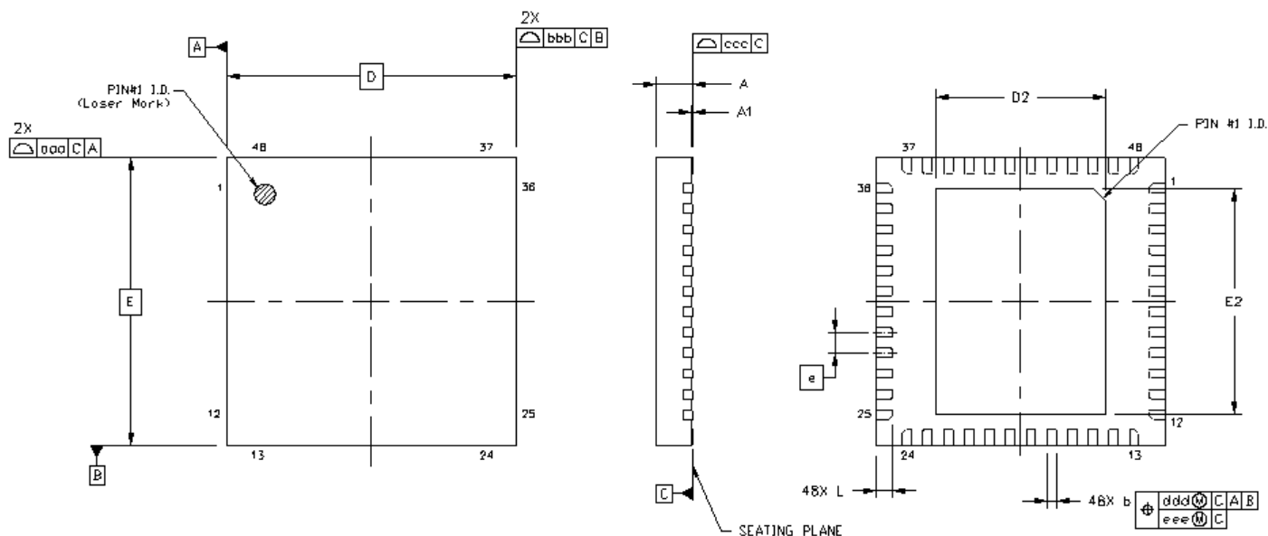
Figure 7.1. 48-Pin QFN Package
