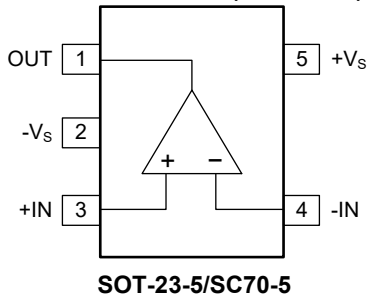
SGM8049-1XN5G SGM8049-1AXC5G (TOP VIEW)
