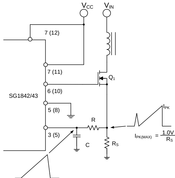
Figure 17 • Current Sense Spike Suppression
