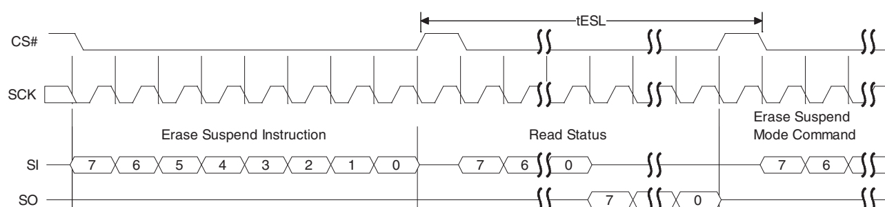
Figure 115. Erase Suspend Command Sequence
