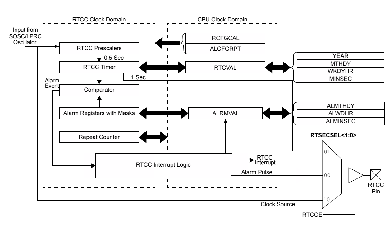
FIGURE 20-1: RTCC BLOCK DIAGRAM
