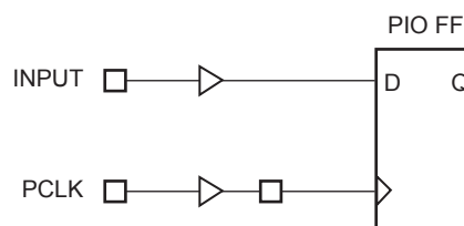
Figure 51. Input to Primary Clock Setup/Hold Time
