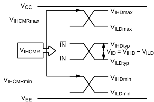
Figure 16. V_{IHCMR} Diagram
