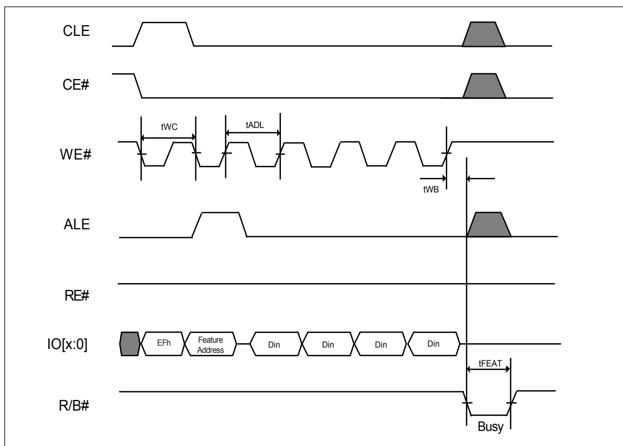
Figure 27. AC Waveforms for Set Feature (ONFI) Operation
