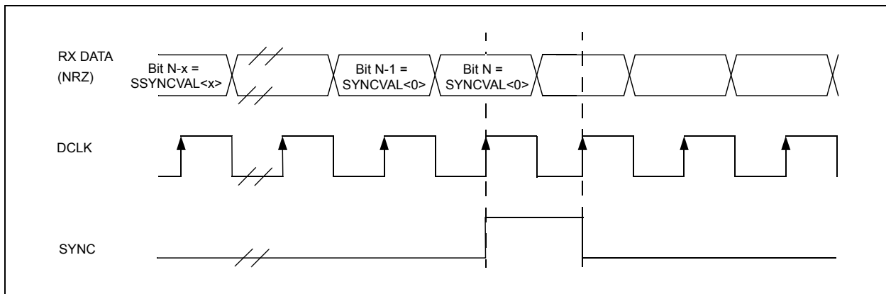
FIGURE 3-15: SYNC WORD RECOGNITION
