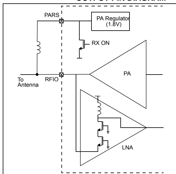
FIGURE 2-3: COMMON RF INPUT AND OUTPUT PIN DIAGRAM
