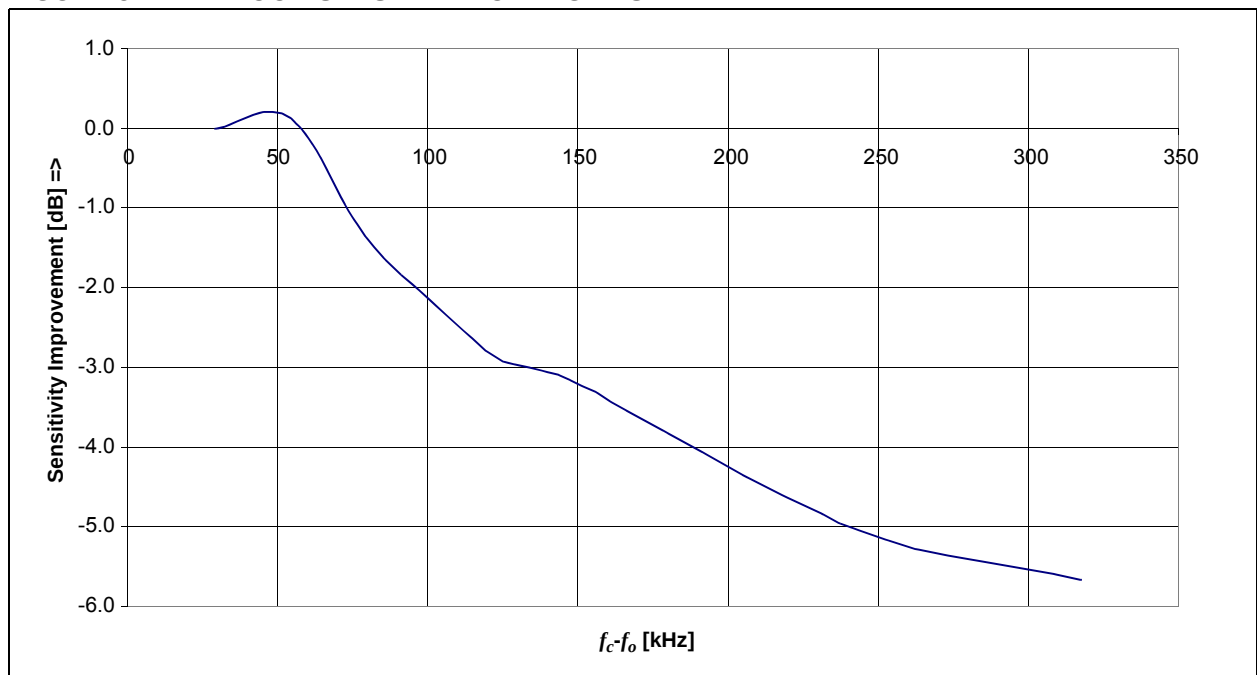
FIGURE 5-11: OOK SENSITIVITY CHANGE VS. RX BW
