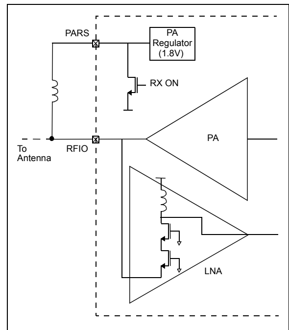
FIGURE 4-6: FRONT-END DESCRIPTION
