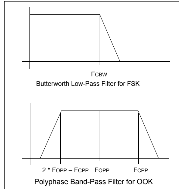
FIGURE 3-5: IF FILTERS IN FSK AND OOK MODES
