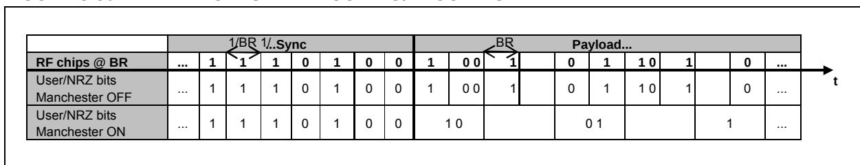
FIGURE 3-30: MANCHESTER ENCODING/DECODING
