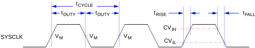
Figure 2. Timing Diagram—SYS_XTAL_IN
