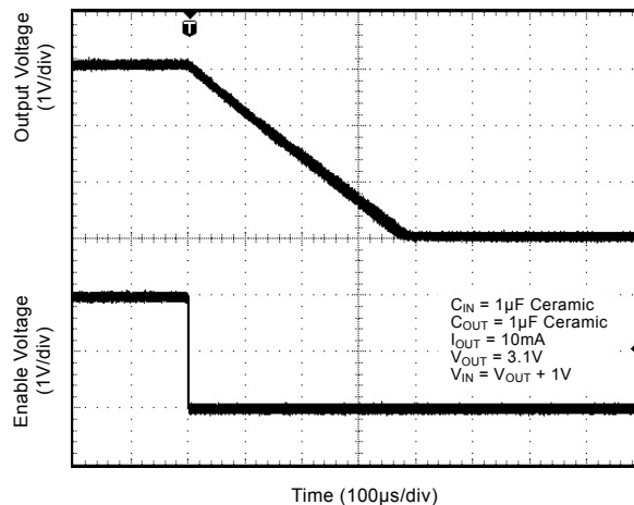
Shutdown Delay
