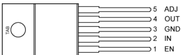
5-Pin TO-220 Adjustable Voltage (T) MIC29152/29302/29502
