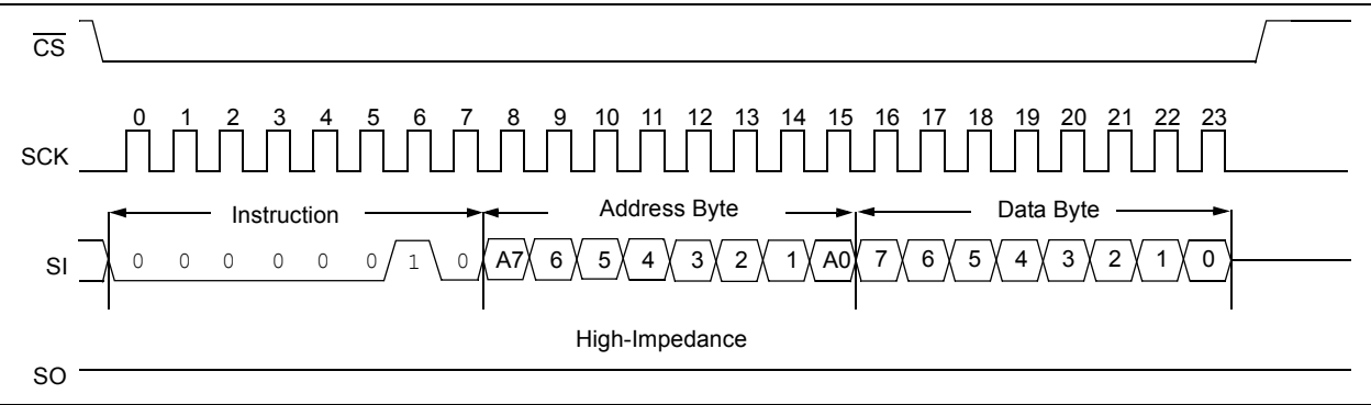
FIGURE 5-4: BYTE WRITE INSTRUCTION
