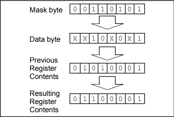
FIGURE 5-1: BIT MODIFY
