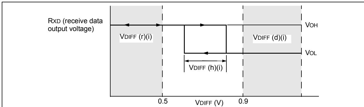
FIGURE 7-6: HYSTERESIS OF THE RECEIVER
