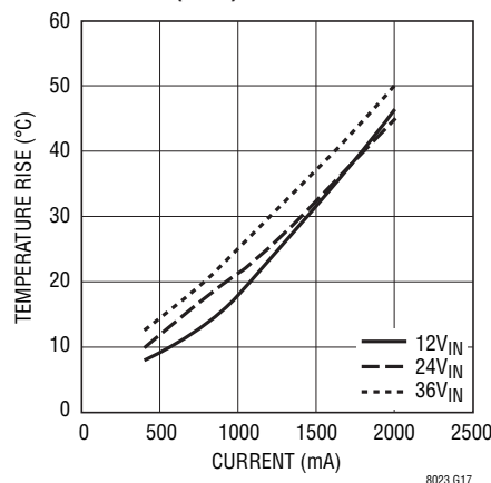
5V OUT Junction Temperature vs Load (LGA)
