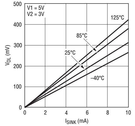
Voltage Output Low vs Output Sink Current ( \overline{RST} , COMP_n )
