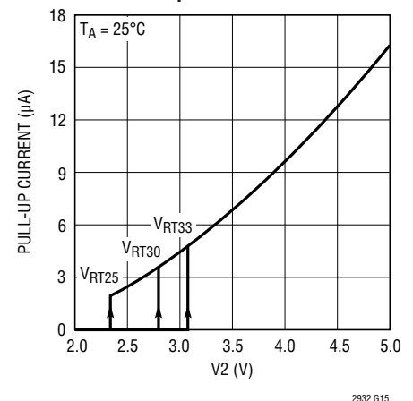
\overline{RST} Pull-Up Current vs V_2
