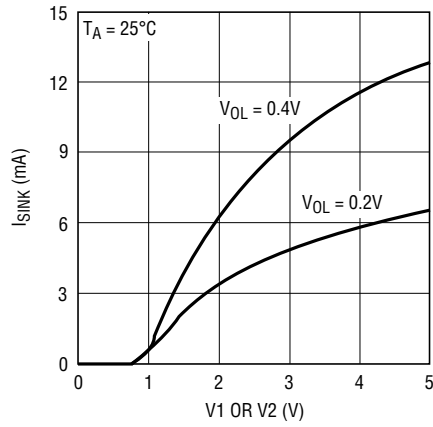
I_{SINK} vs Supply Voltage ( \overline{RST} , COMP_n )
