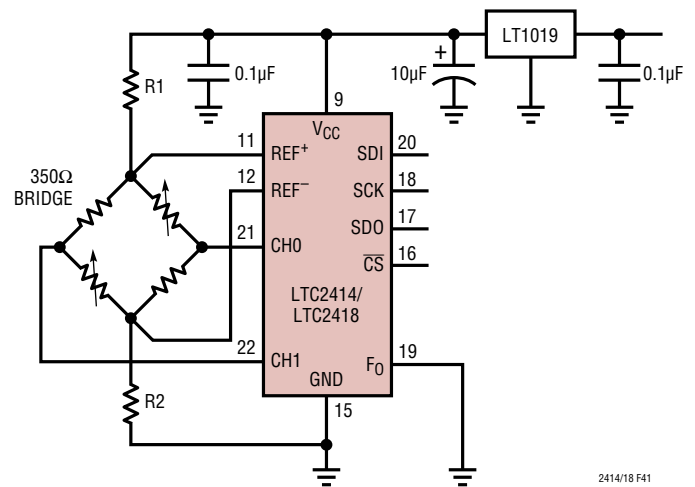
Figure 41. Simple Bridge Connection
