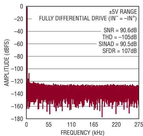
Figure 7c. IN + /IN - = 450mV 200Hz Fully Differential Sine, 0V ≤ V CM ≤ 24V, 32k Point FFT, f SMPL = 550kps. Circuit Shown in Figure 7a
