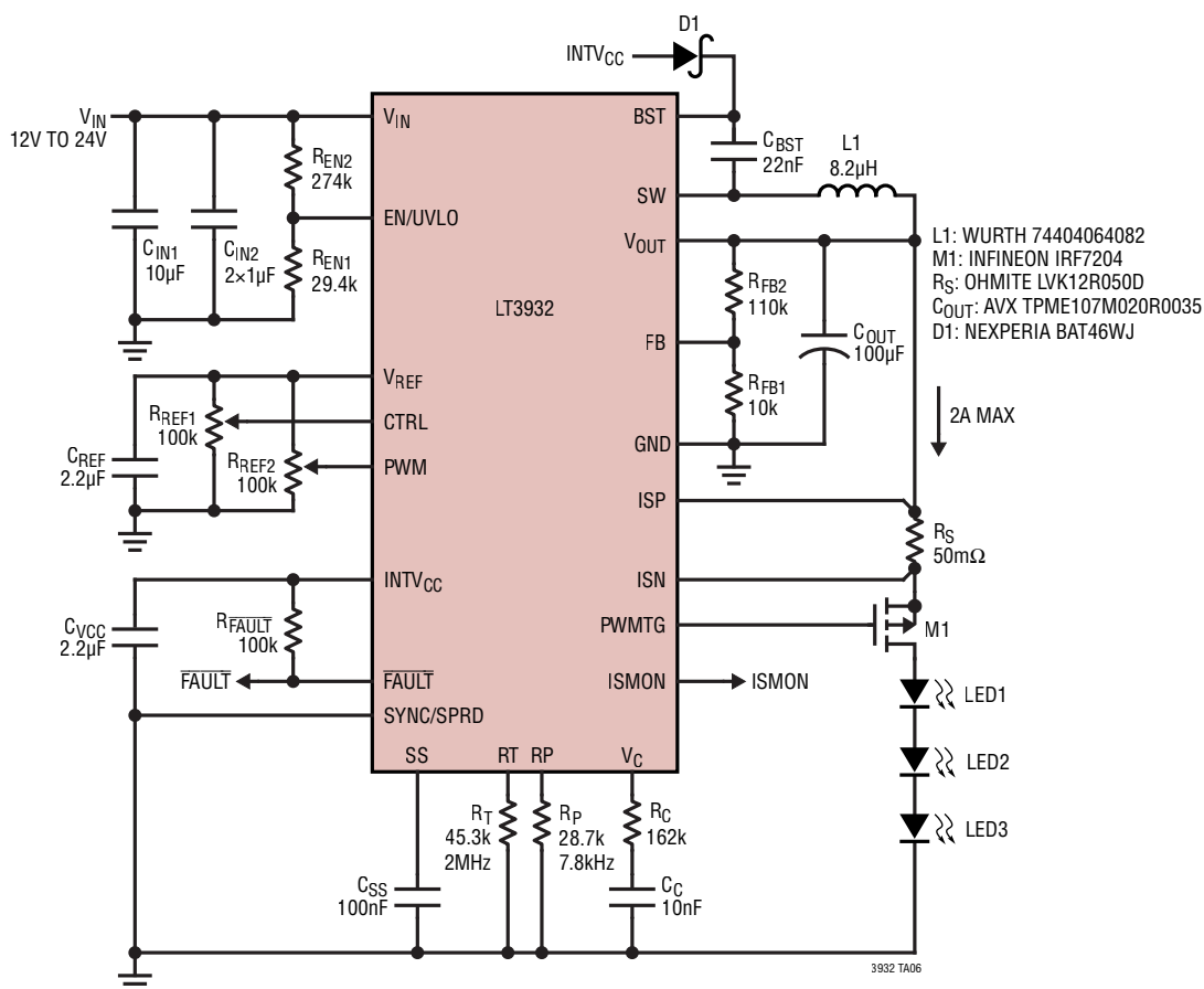
2A LED Driver with Internal PWM Dimming
