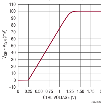
LED Current (Analog CTRL)
