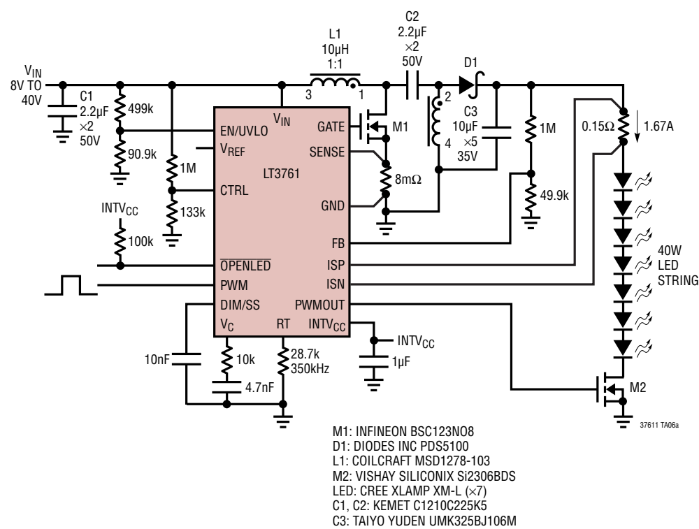
40W SEPIC LED Driver
