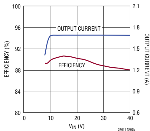
SEPIC Efficiency, Output Current vs V_{IN}
