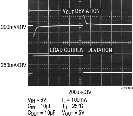
Transient Response, C_{BYP} = 0\text{pF}
