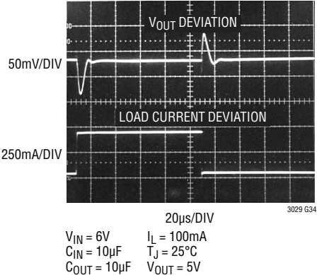
Transient Response, C_{BYP} = 0.01\mu\text{F}
