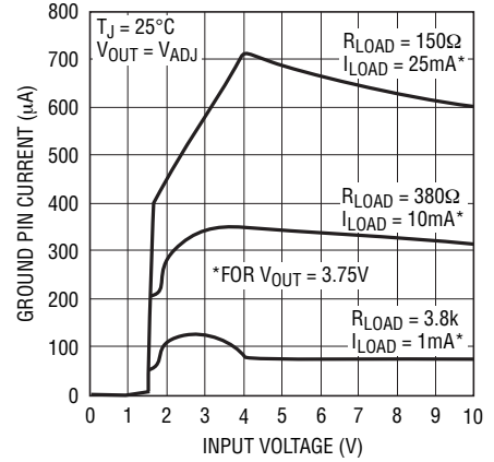
LT1121 Ground Pin Current
