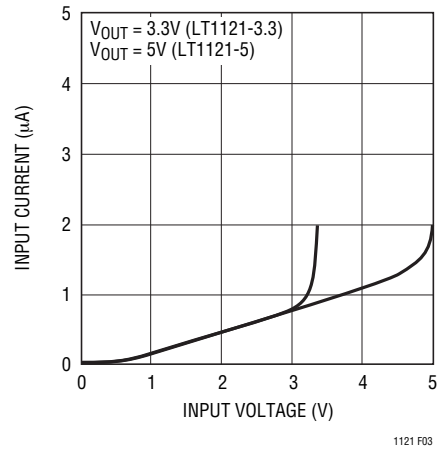
Figure 3. Input Current
