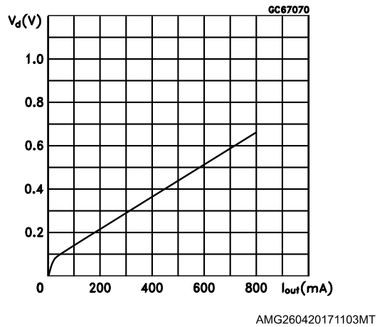
Figure 4: Dropout voltage vs output current
