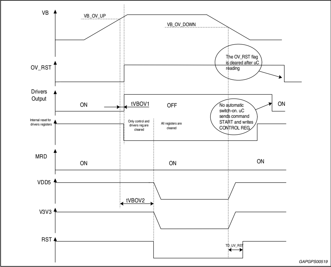
Figure 18. VB overvoltage diagram
