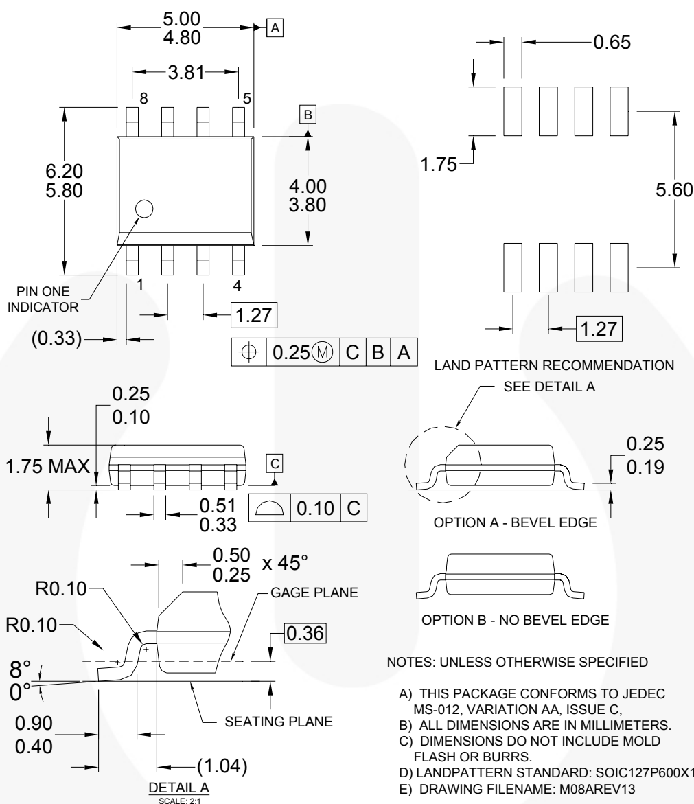
Figure 45. 8-Lead Small Outline Package (SOP)
